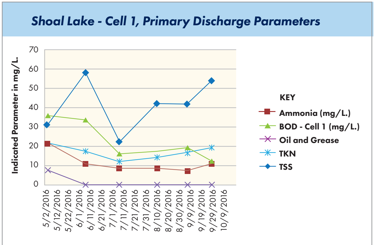
Fig.1: Operating results for Shoal Lake Cell #1.
