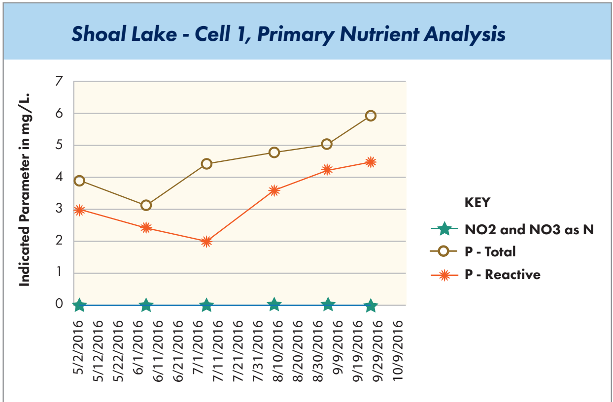
Fig. 2: Shoal Lake Cell #1 Nutrient Data
