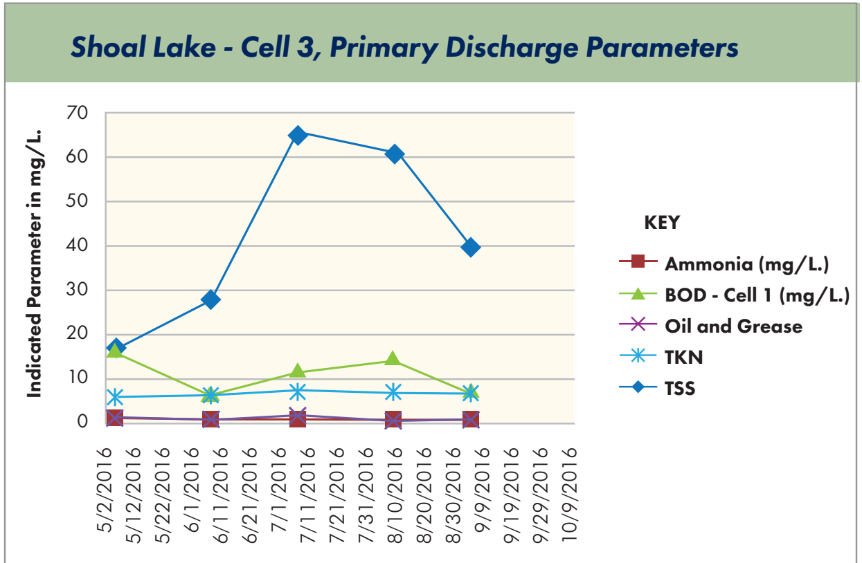
Fig. 5: Shoal Lake Cell #3 performance data.
